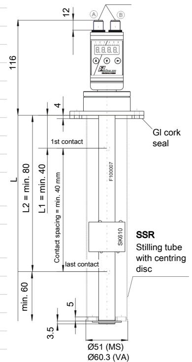
Housing swivels 270°
