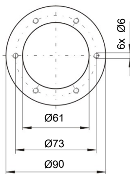
Flange drawing
